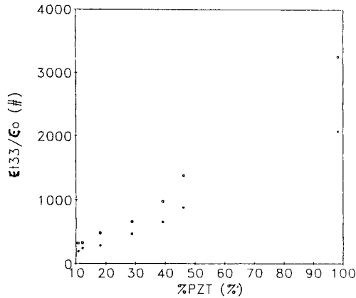
Figure 2. The dielectric constant of 1-3 PZT-polymer composites with silver epoxy and evaporated silver electrodes.
