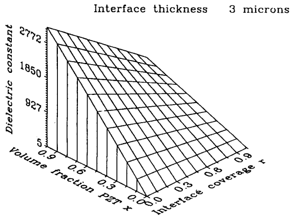
Figure 5. Theoretical values of the dielectric constant as a function of PZT-binder interface area, r , and as a function of the PZT percentage, x , in the composite. (See text for values assumed in the calculations).
