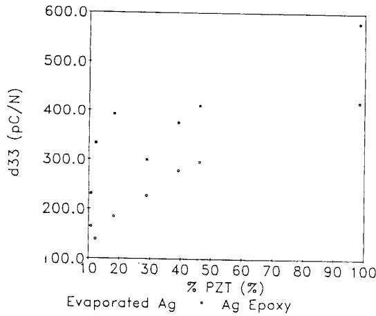
Figure 8. The hydrostatic charge coefficient, d_{33} , of 1-3 PZT-polymer composites with silver epoxy and evaporated silver electrodes.
